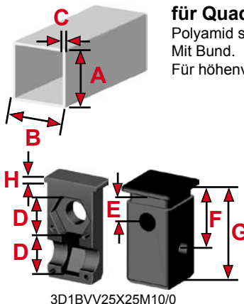
3D1BVV25X25M10/0
