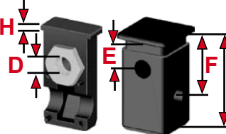
3D1BV25X25M10/1
