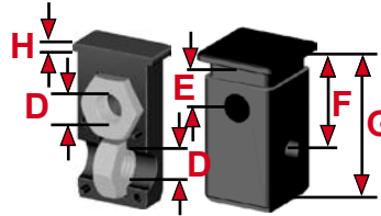
3D1BVV25X25M10/2
