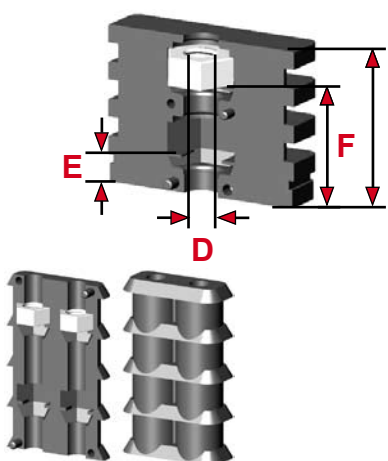
1D1V30X15X1.5M5/1H+1H
